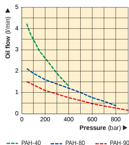
FLOW CHART
