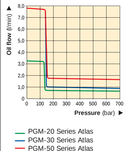
FLOW CHART
